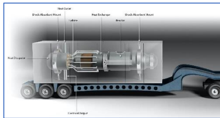
DOE MARVEL Microreactor
